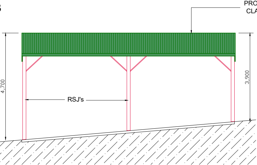
EAST ELEVATION
