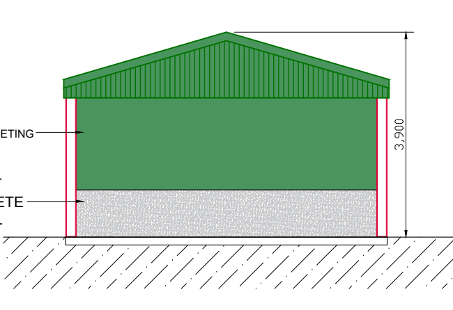
NORTH ELEVATION
