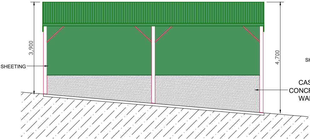
WEST ELEVATION
